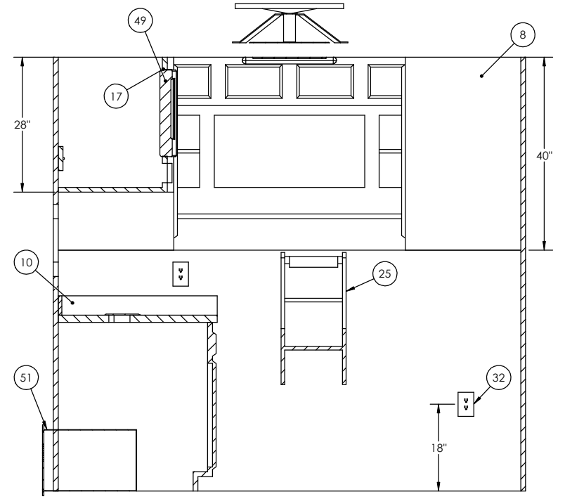
SECTION E-E
