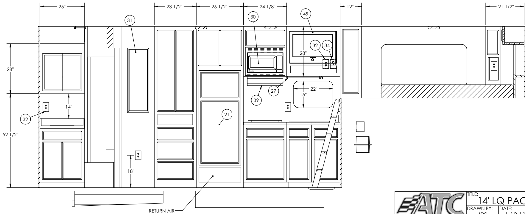
ROAD SIDE SECTION B-B
