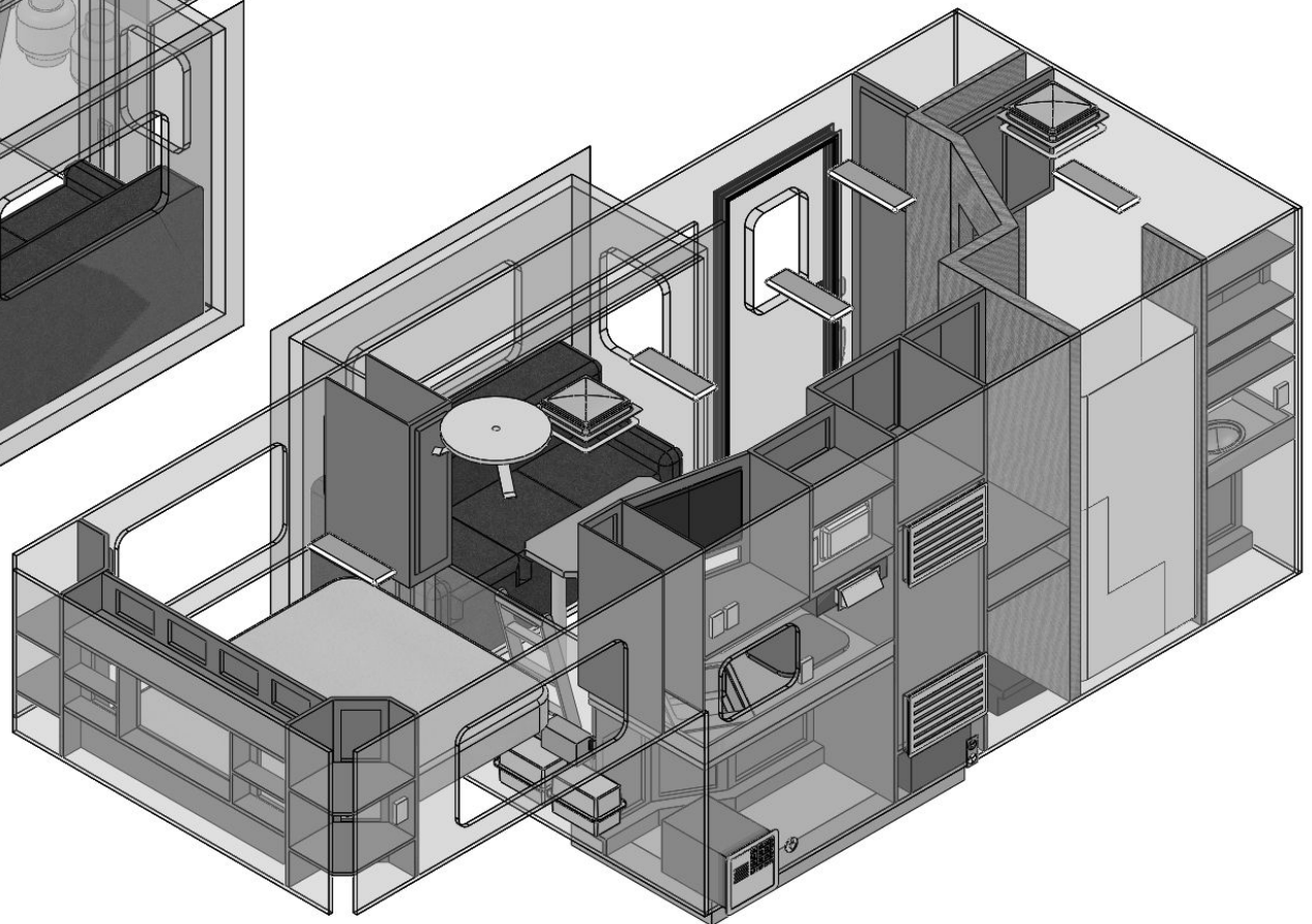
ROAD SIDE VIEW
